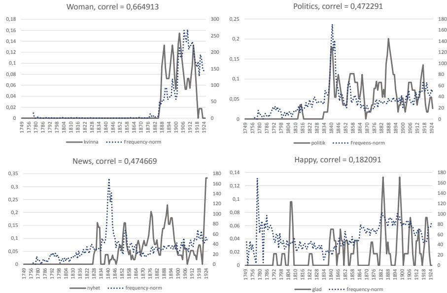
Fig. 2. Smoothened Jaccard similarities plotted against the normalized frequency of each word. The Jaccard similarity is on the primary axis (on the left-hand side) and the normalized frequencies on the secondary axis.
